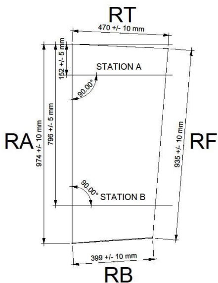
RUDDER DIMENSIONS AND STATIONS
